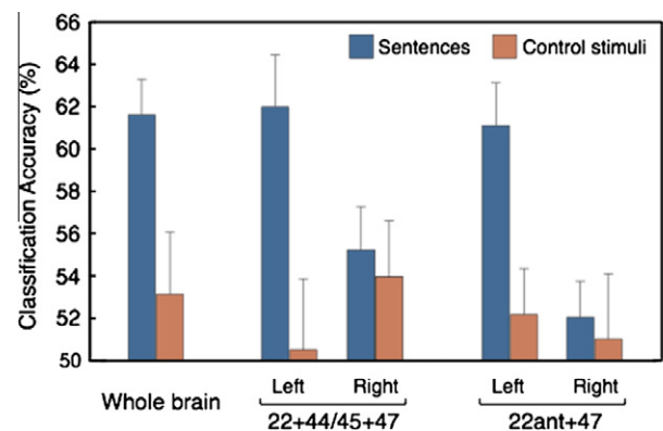
Fig. 2. Classification results within the whole brain, the union of all ROIs of interest (complete BA22 + BA47 + BA44/45), and the union of aBA22 + 47 in the left and right hemispheres. Bars indicate standard error.
