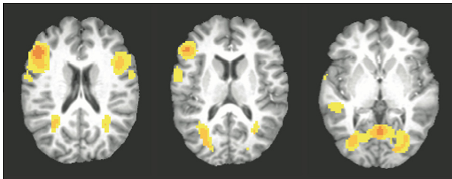
Fig. 4. GLM analysis of sentence condition – rest. Activation includes areas in BA22, and BA44/45. BA47 showed deactivation (not pictured) to the sentence condition – rest ( \alpha = 0.05 ).
